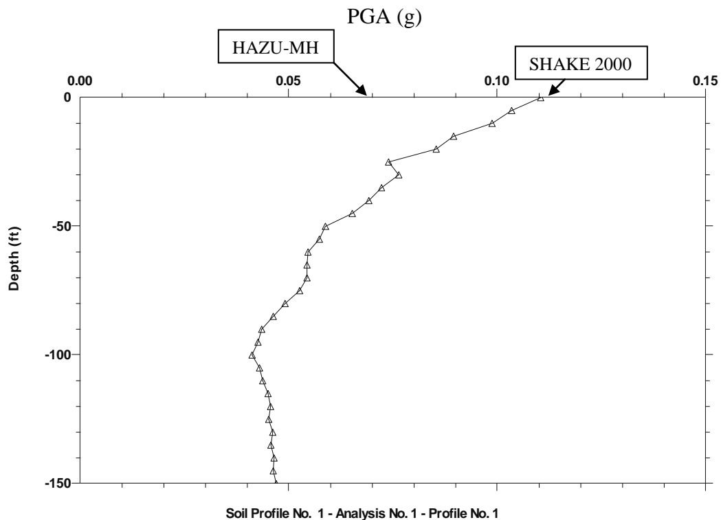
Figure 5.4. SHAKE 2000 PGA Output for St. Charles Smartt Airport
