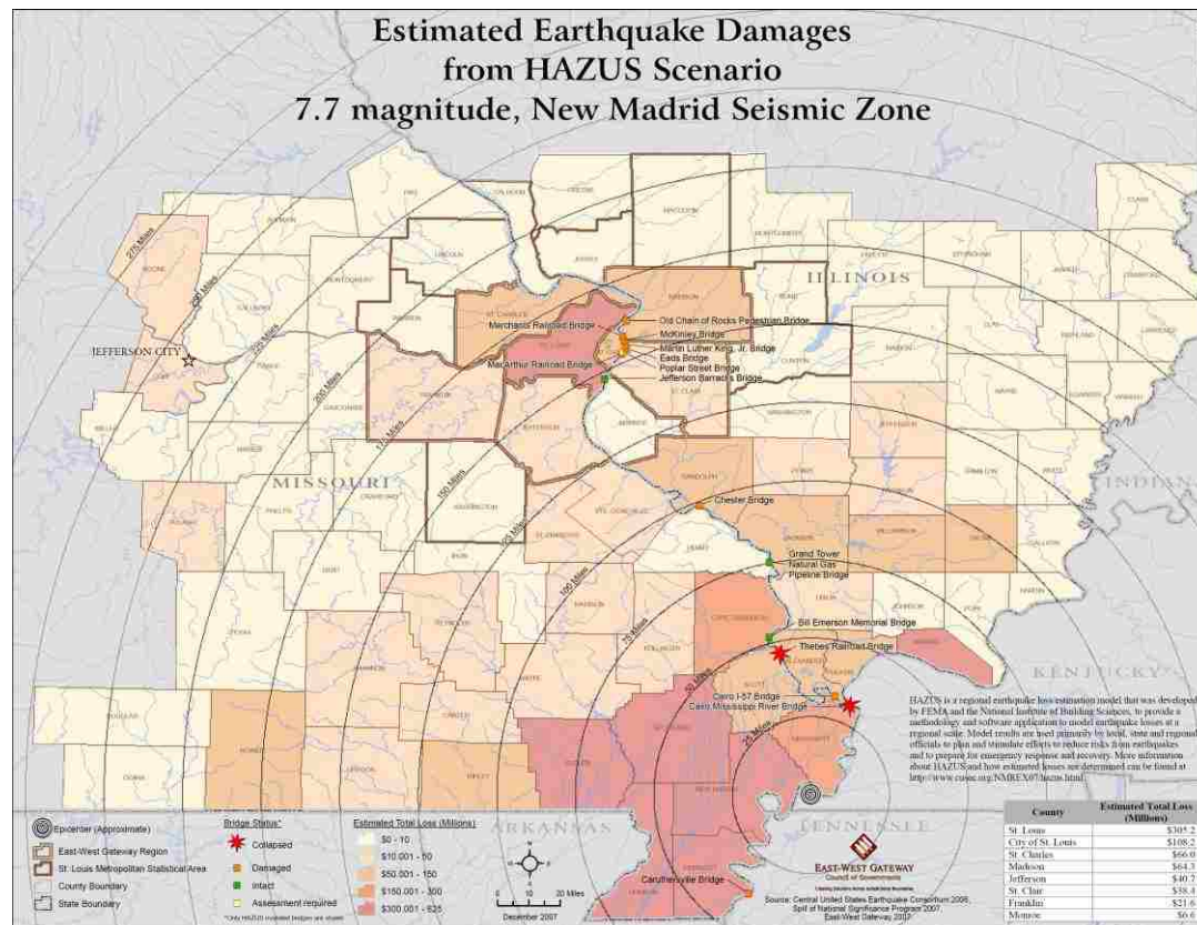
Figure 3.2. East-West Gateway HAZUS-MH Study Results
