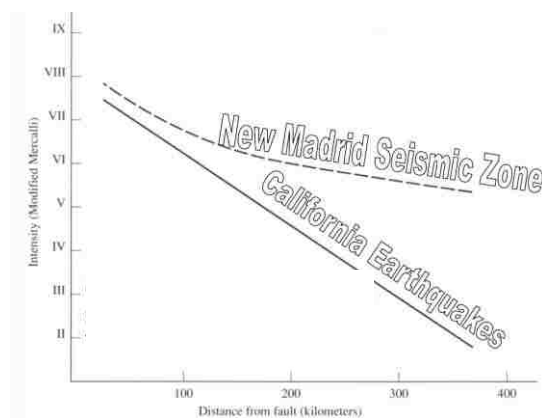
Figure 4.4. Comparison of Earthquake Intensity vs. Distance
