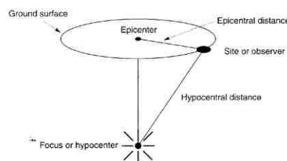
Figure 4.1. Earthquake Terminology (Source: Kramer 1996, page 43)
