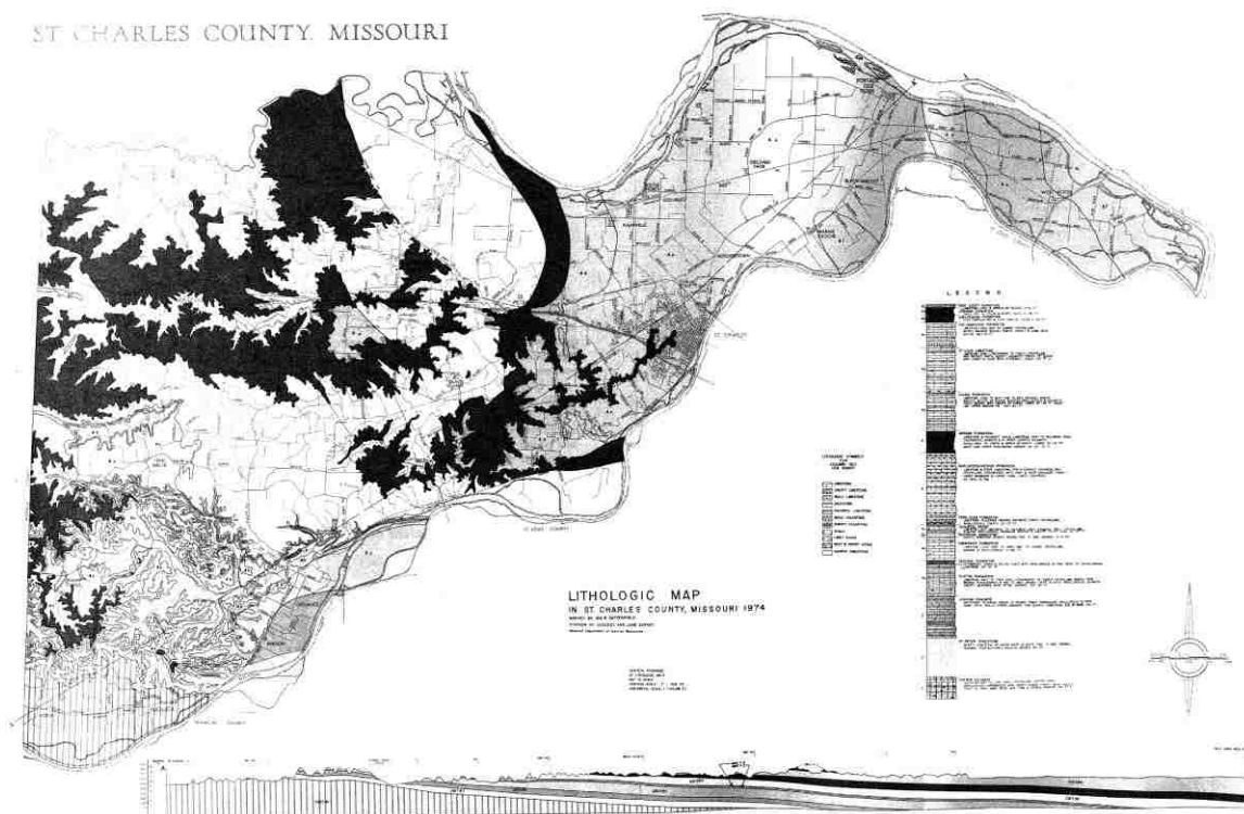
Figure 2.4. St. Charles County Lithologic Map (Source: Missouri Geologic Survey 1977, pages 149-150)
