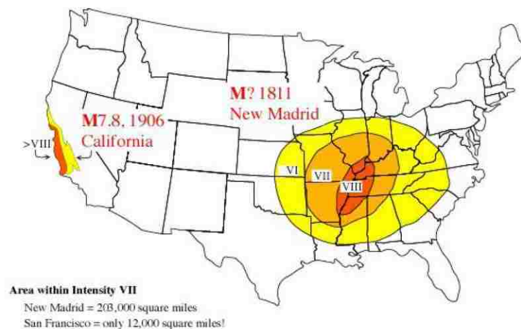
Figure 4.3. Comparison of Earthquake Influence Across the Country
